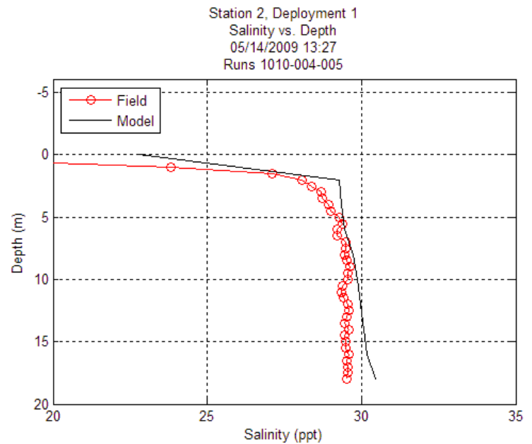
Figure E-2c Comparison of Predicted and Observed Salinity Profiles, Site 2 Sediment Transport Evaluation Report East Waterway Operable Unit
